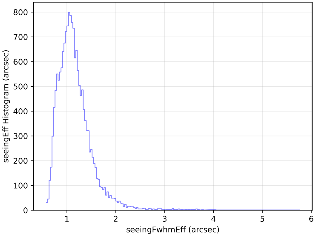
too_elab_r32_d2_gz_v3.4_10yrs Yr 1 u band: seeingEff Histogram
