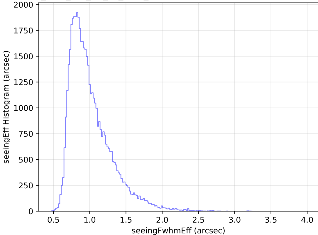
too_elab_r32_d2_gz_v3.4_10yrs Yr 1 r band: seeingEff Histogram
