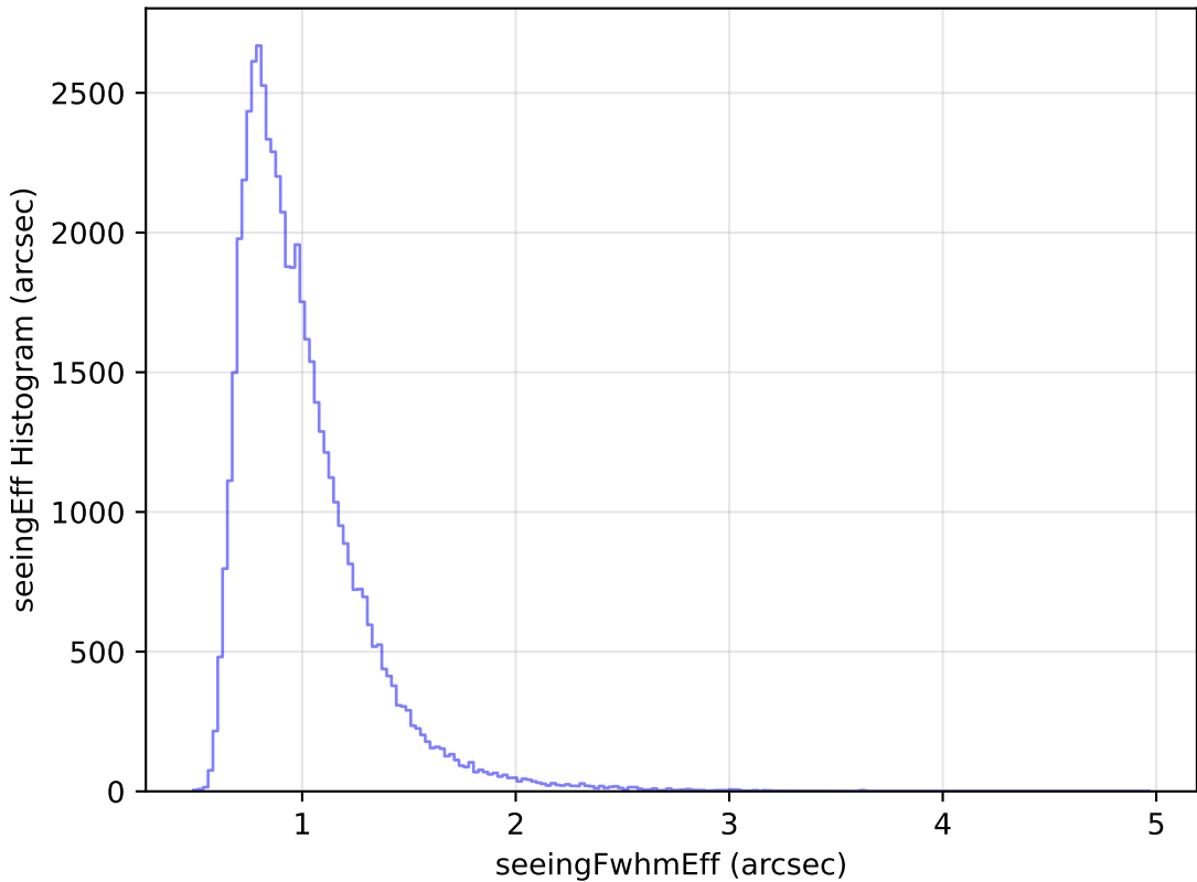
too_elab_r32_d2_gz_v3.4_10yrs Yr 1 i band: seeingEff Histogram
