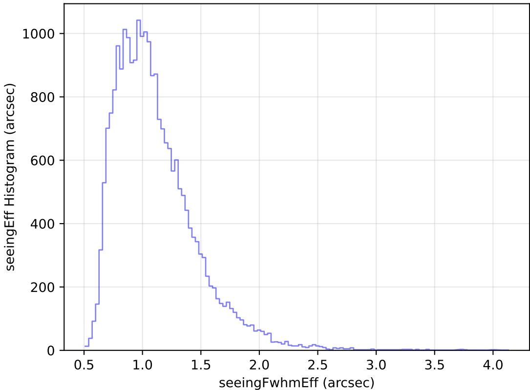
too_elab_r32_d2_gz_v3.4_10yrs Yr 1 g band: seeingEff Histogram
