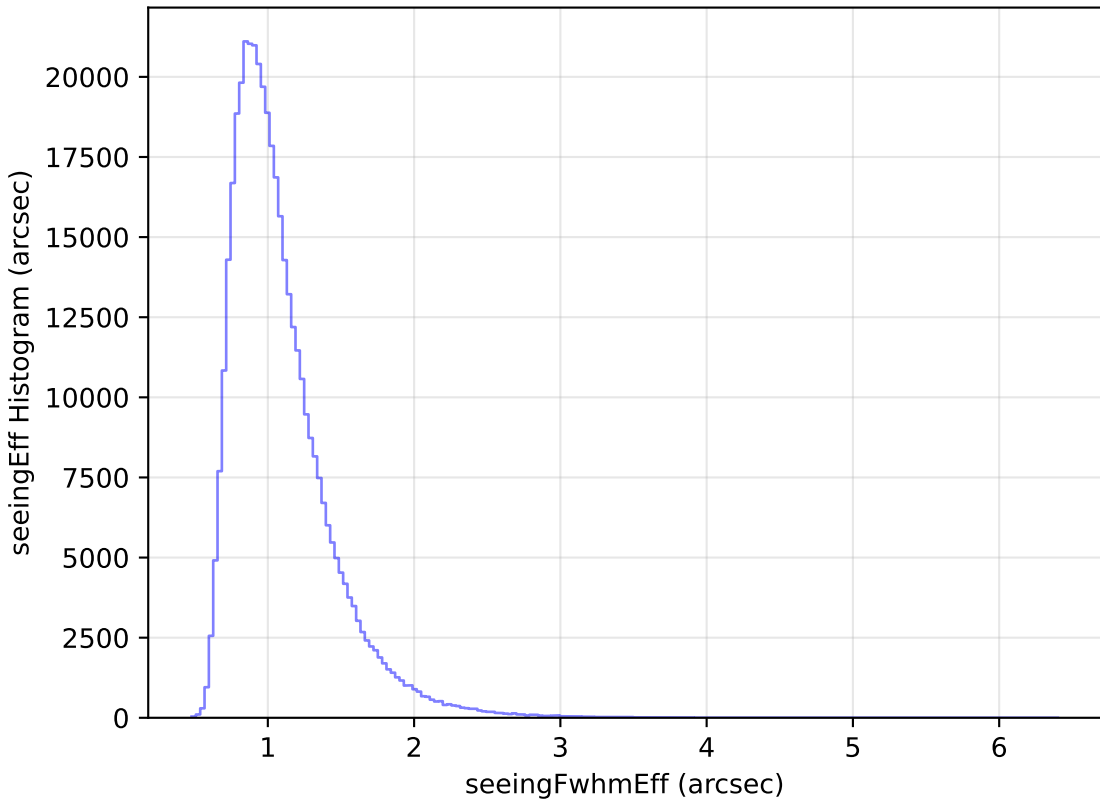
too_elab_r32_d2_gz_v3.4_10yrs WFD z band: seeingEff Histogram
