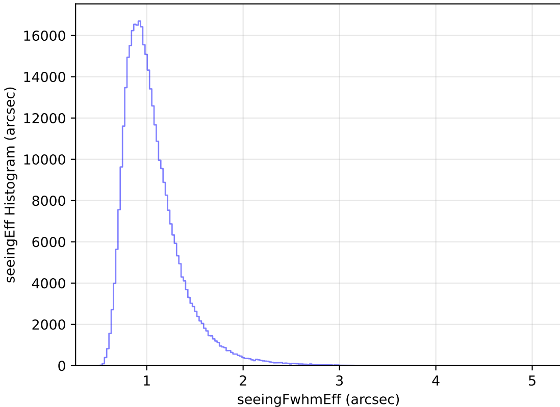
too_elab_r32_d2_gz_v3.4_10yrs WFD y band: seeingEff Histogram
