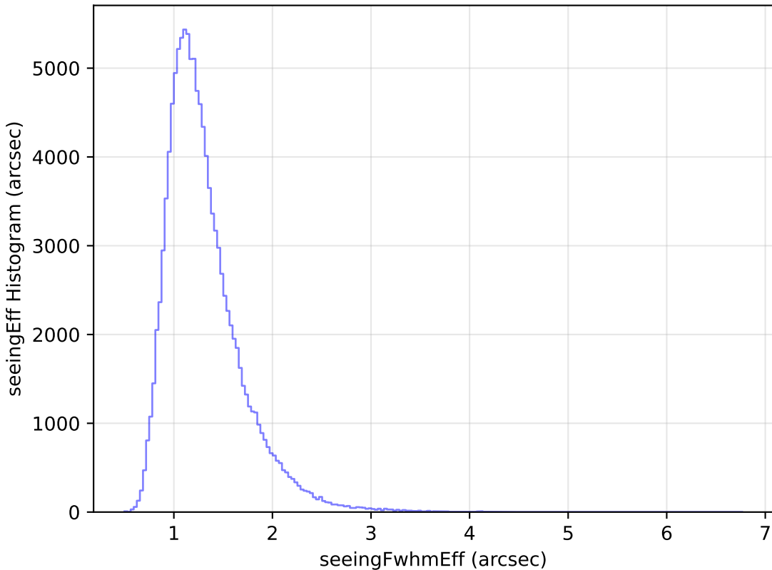
too_elab_r32_d2_gz_v3.4_10yrs WFD u band: seeingEff Histogram
