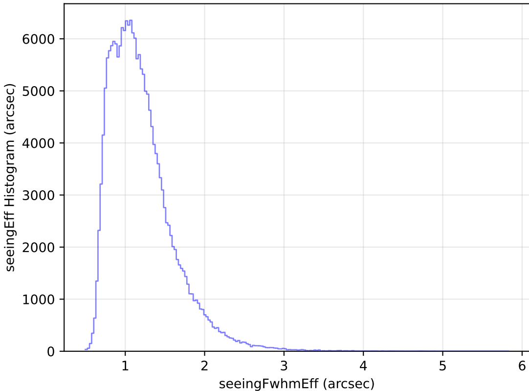
too_elab_r32_d2_gz_v3.4_10yrs WFD g band: seeingEff Histogram
