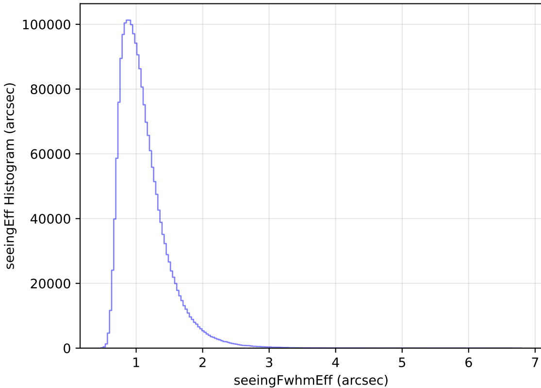
too_elab_r32_d2_gz_v3.4_10yrs WFD all bands: seeingEff Histogram
