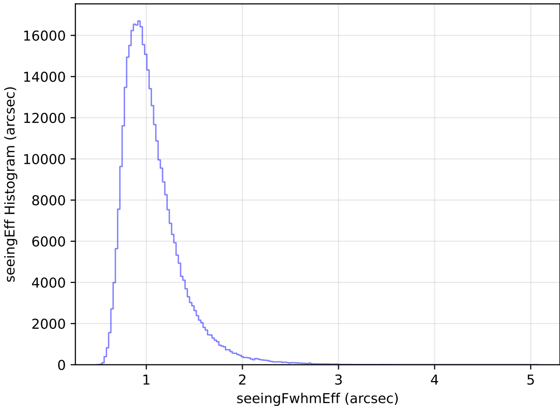
too_elab_r32_d2_gz_v3.4_10yrs All sky y band: seeingEff Histogram
