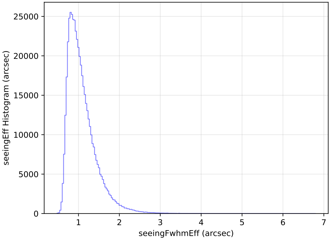
too_elab_r32_d2_gz_v3.4_10yrs All sky i band: seeingEff Histogram
