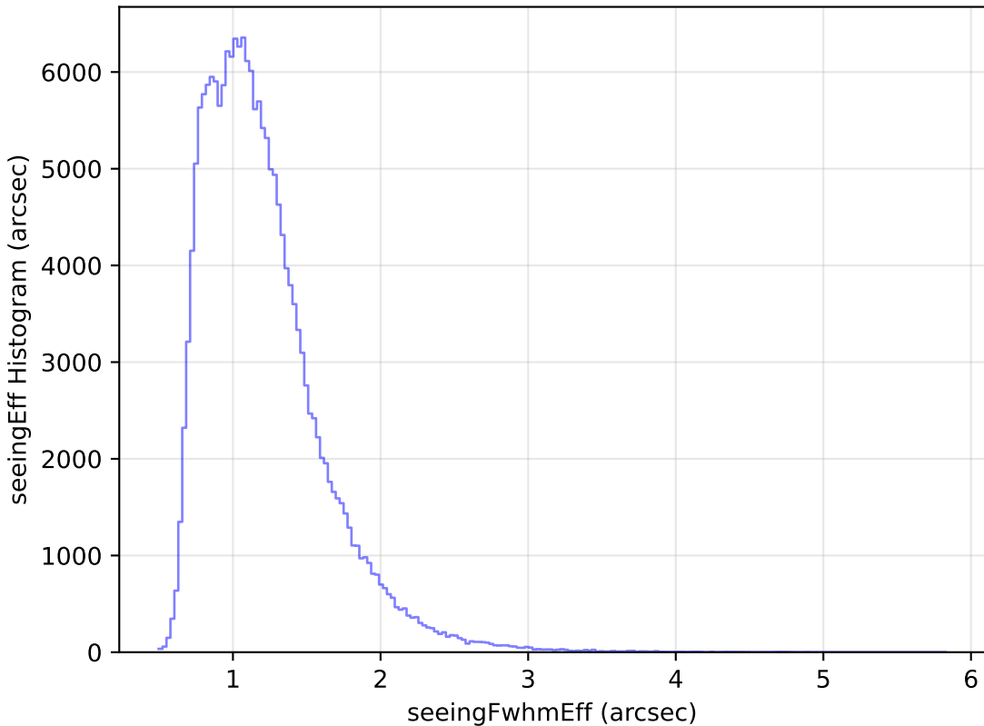
too_elab_r32_d2_gz_v3.4_10yrs All sky g band: seeingEff Histogram
