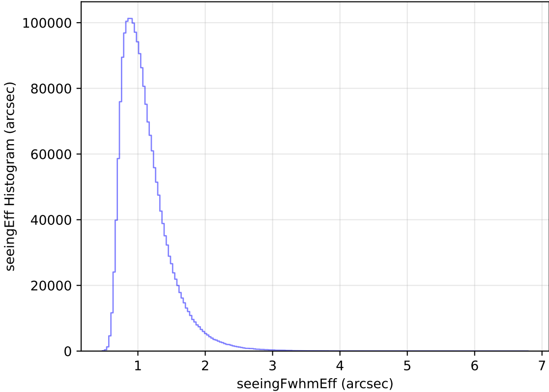
too_elab_r32_d2_gz_v3.4_10yrs All sky all bands: seeingEff Histogram
