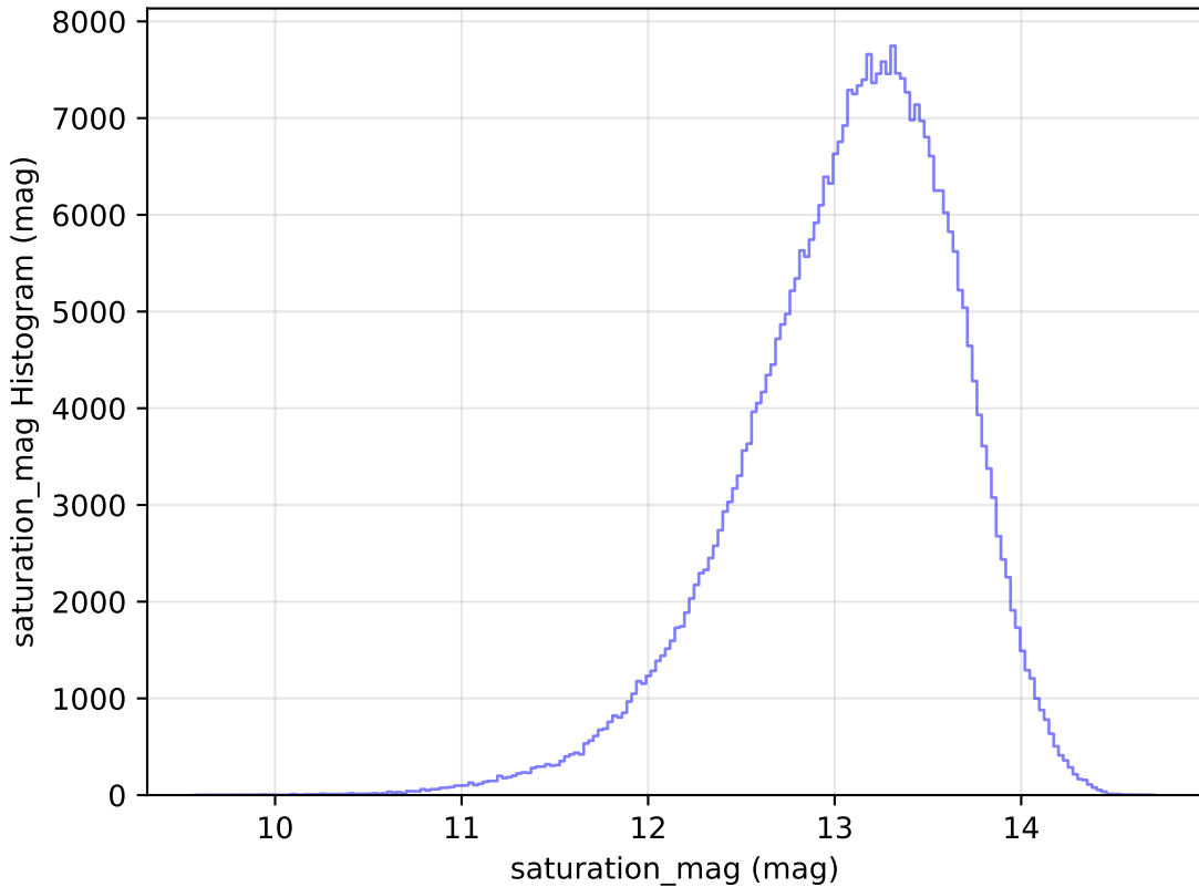
too_elab_r32_d2_gz_v3.4_10yrs WFD y band: saturation_mag Histogram
