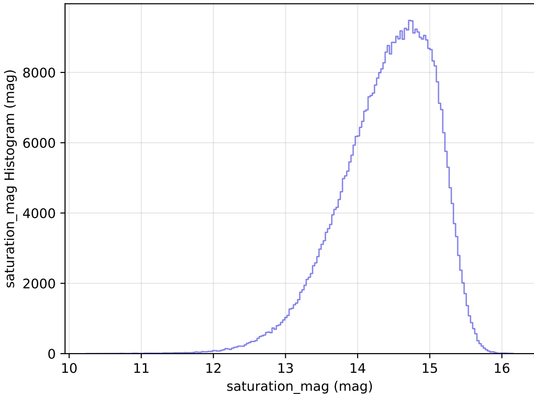
too_elab_r32_d2_gz_v3.4_10yrs WFD i band: saturation_mag Histogram
