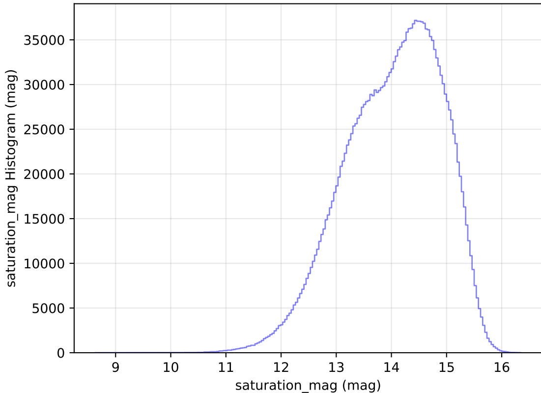
too_elab_r32_d2_gz_v3.4_10yrs WFD all bands: saturation_mag Histogram
