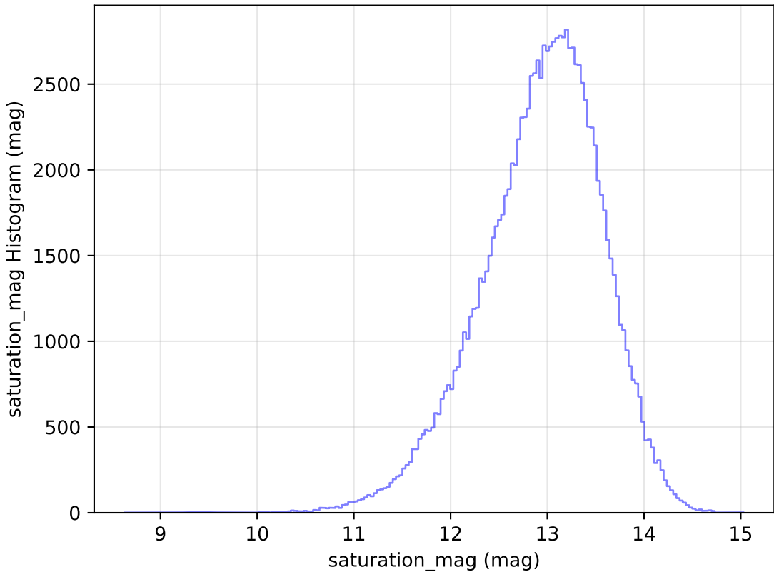
too_elab_r32_d2_gz_v3.4_10yrs All sky u band: saturation_mag Histogram
