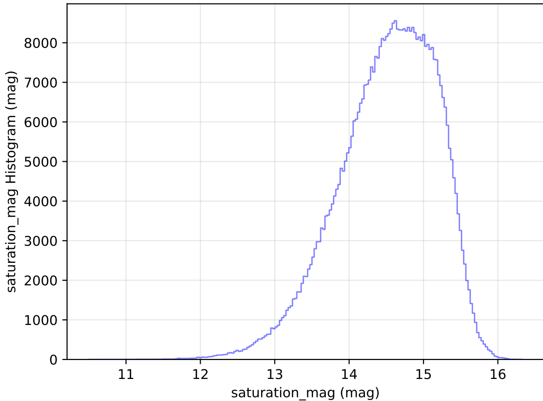
too_elab_r32_d2_gz_v3.4_10yrs All sky r band: saturation_mag Histogram
