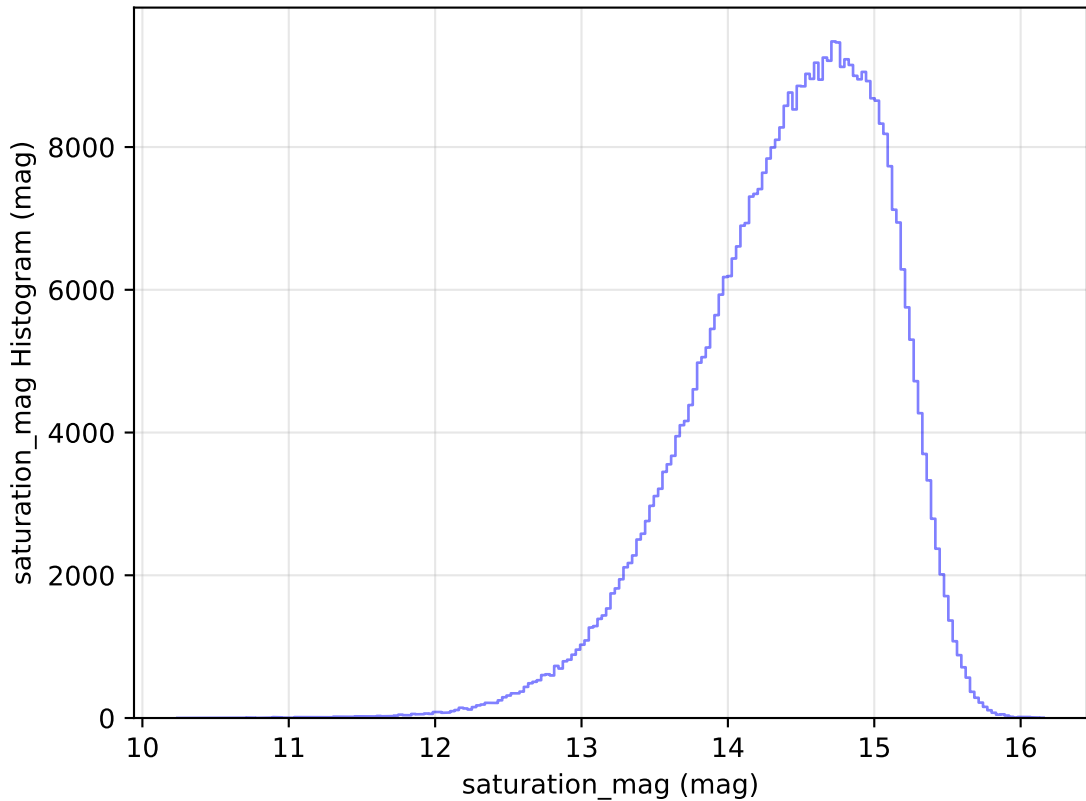
too_elab_r32_d2_gz_v3.4_10yrs All sky i band: saturation_mag Histogram
