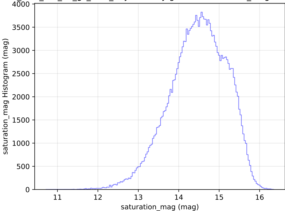
too_elab_r32_d2_gz_v3.4_10yrs All sky g band: saturation_mag Histogram
