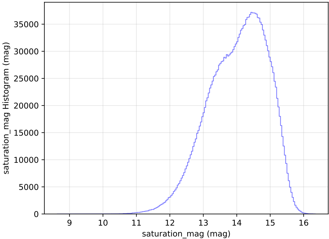
too_elab_r32_d2_gz_v3.4_10yrs All sky all bands: saturation_mag Histogram
