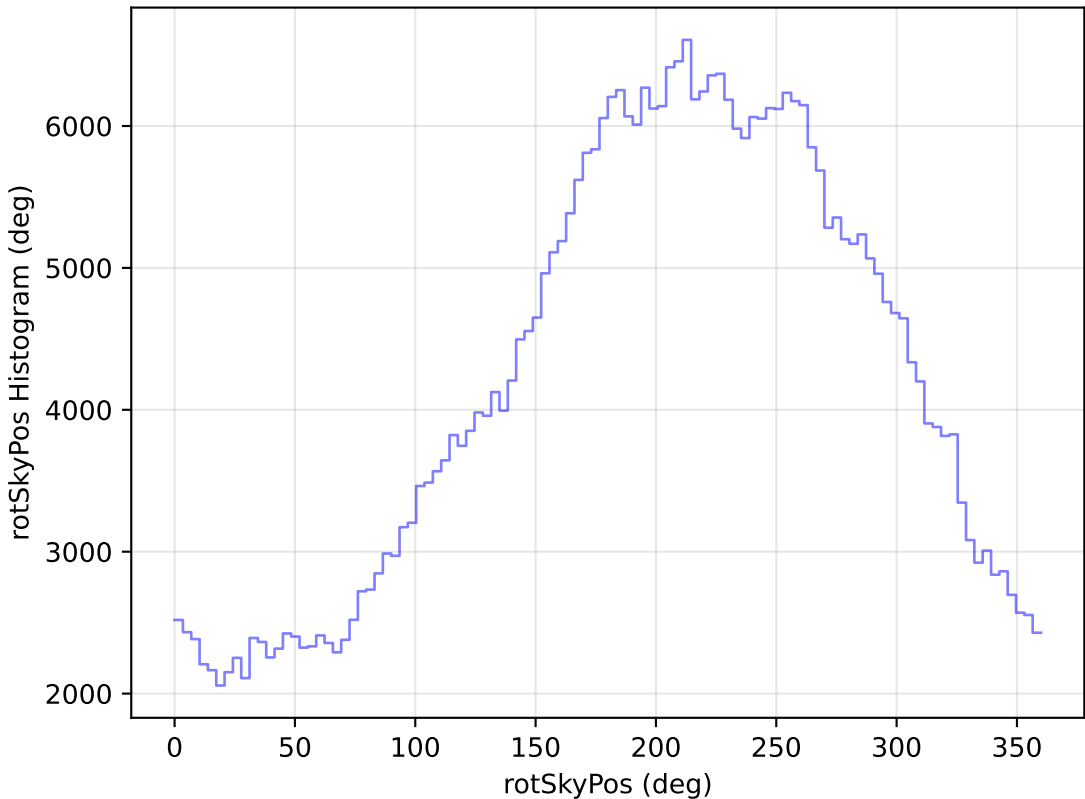
too_elab_r32_d2_gz_v3.4_10yrs WFD z band: rotSkyPos Histogram
