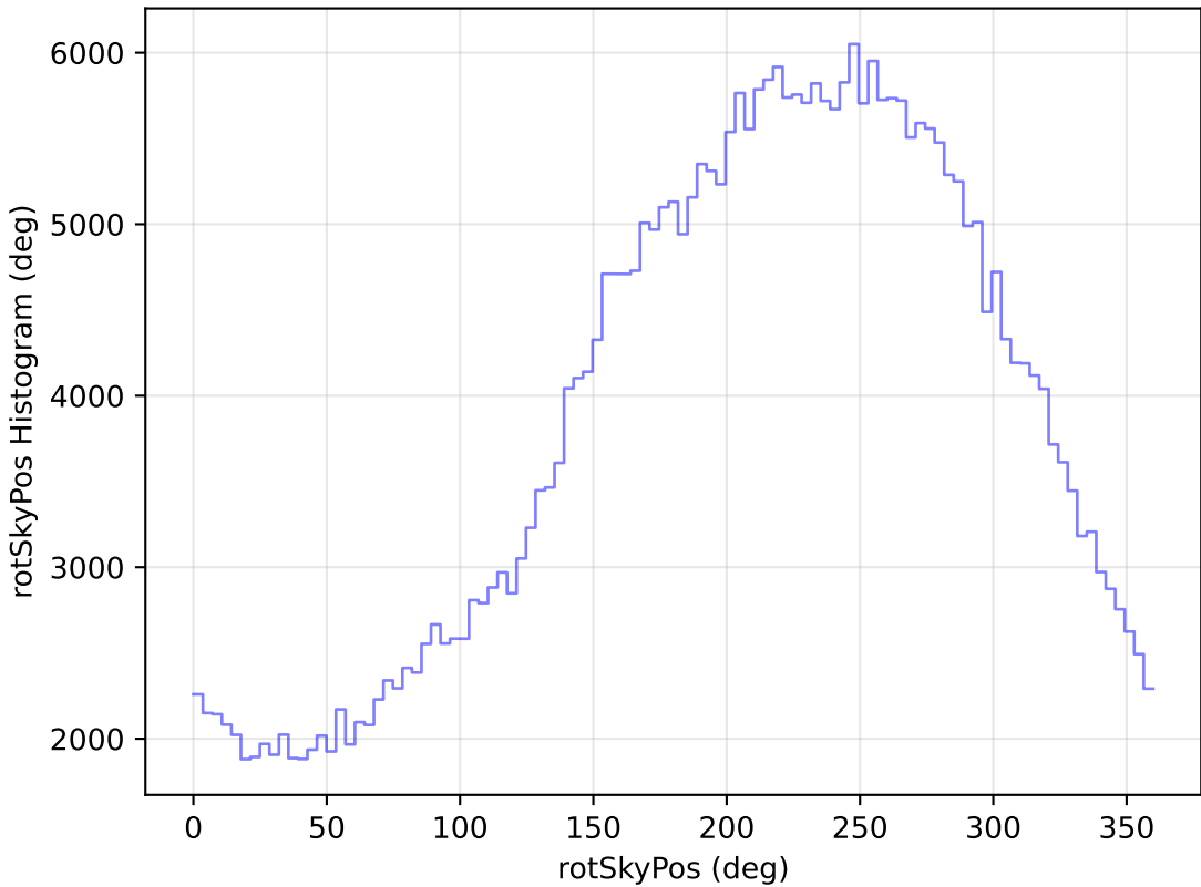
too_elab_r32_d2_gz_v3.4_10yrs WFD y band: rotSkyPos Histogram
