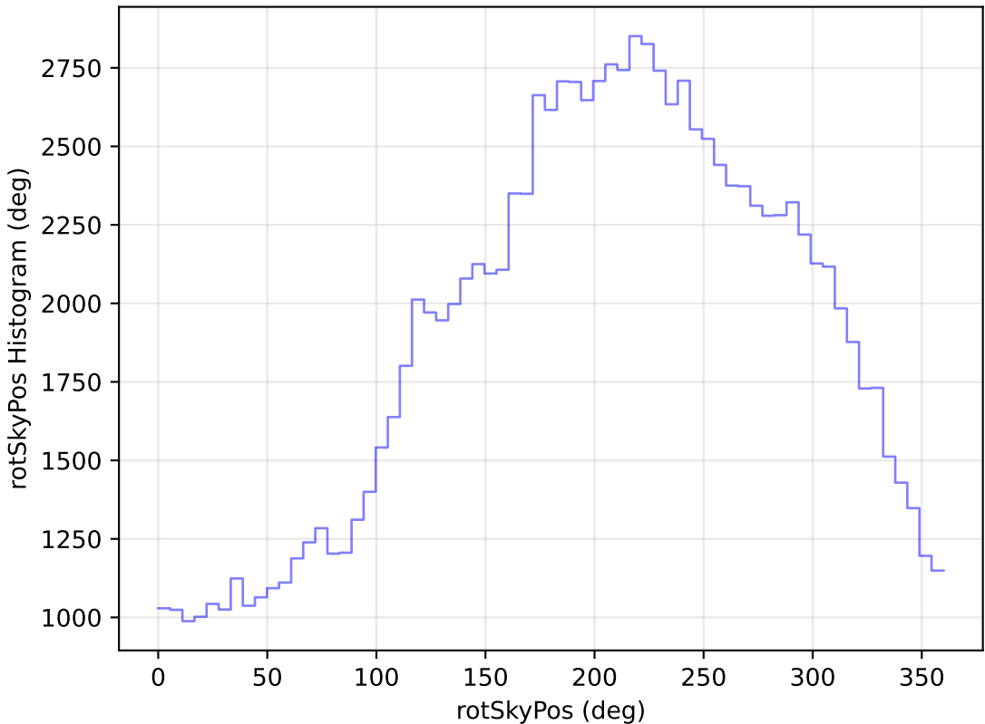
too_elab_r32_d2_gz_v3.4_10yrs WFD u band: rotSkyPos Histogram
