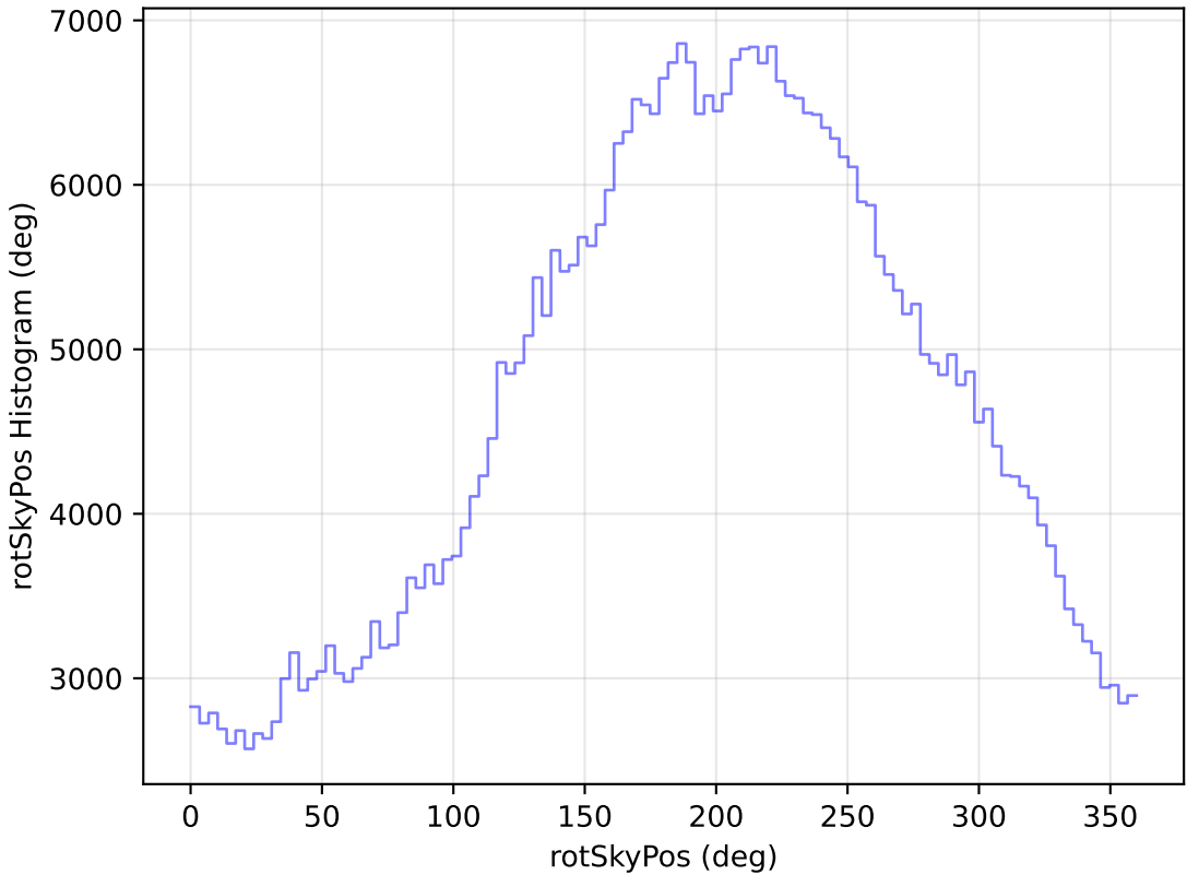
too_elab_r32_d2_gz_v3.4_10yrs WFD r band: rotSkyPos Histogram
