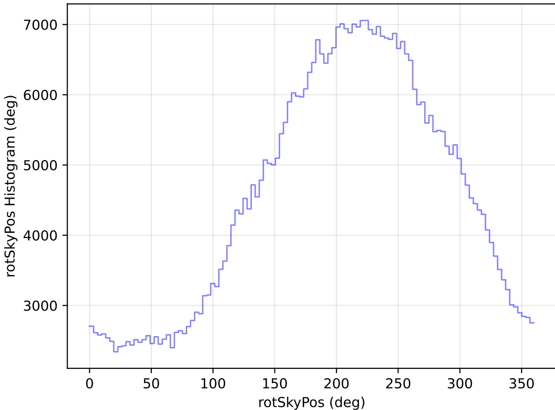
too_elab_r32_d2_gz_v3.4_10yrs WFD i band: rotSkyPos Histogram
