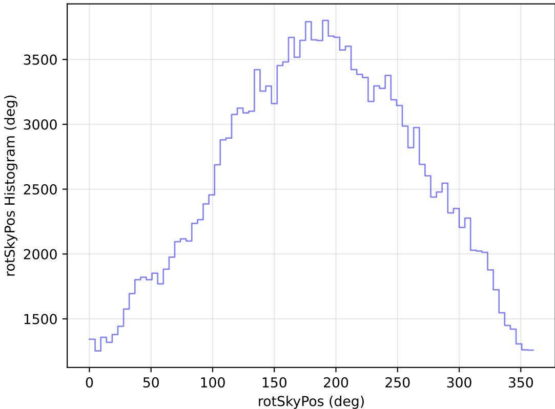
too_elab_r32_d2_gz_v3.4_10yrs WFD g band: rotSkyPos Histogram
