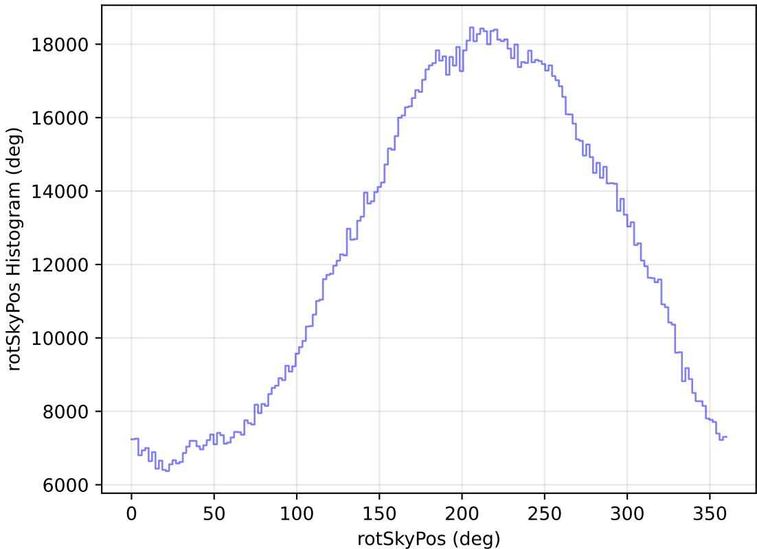
too_elab_r32_d2_gz_v3.4_10yrs WFD all bands: rotSkyPos Histogram
