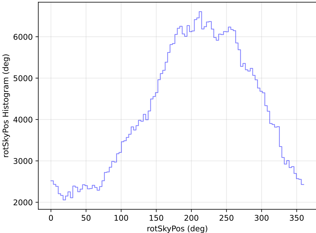
too_elab_r32_d2_gz_v3.4_10yrs All sky z band: rotSkyPos Histogram
