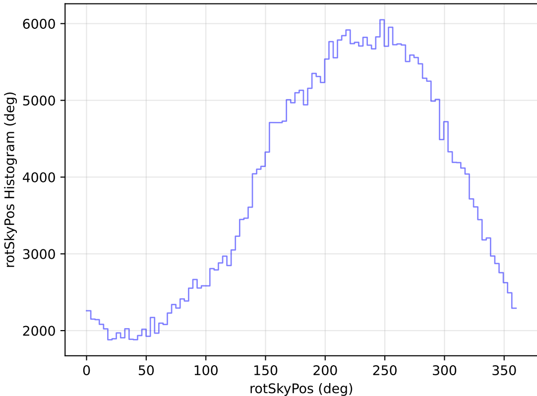
too_elab_r32_d2_gz_v3.4_10yrs All sky y band: rotSkyPos Histogram
