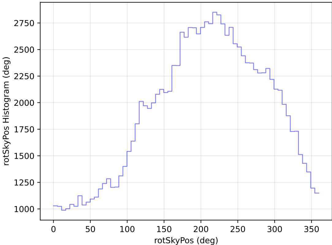
too_elab_r32_d2_gz_v3.4_10yrs All sky u band: rotSkyPos Histogram
