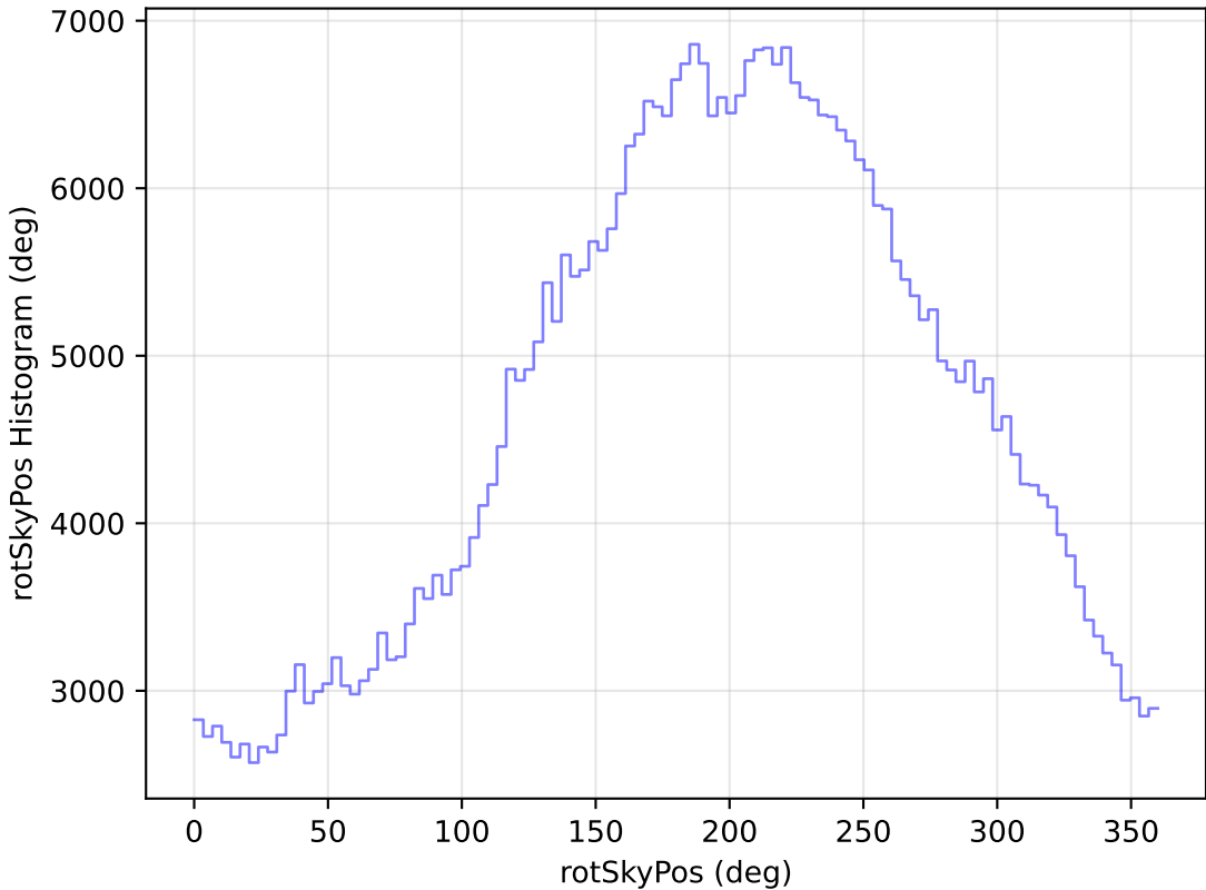
too_elab_r32_d2_gz_v3.4_10yrs All sky r band: rotSkyPos Histogram
