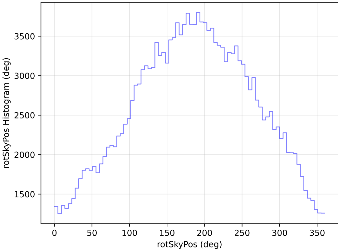
too_elab_r32_d2_gz_v3.4_10yrs All sky g band: rotSkyPos Histogram
