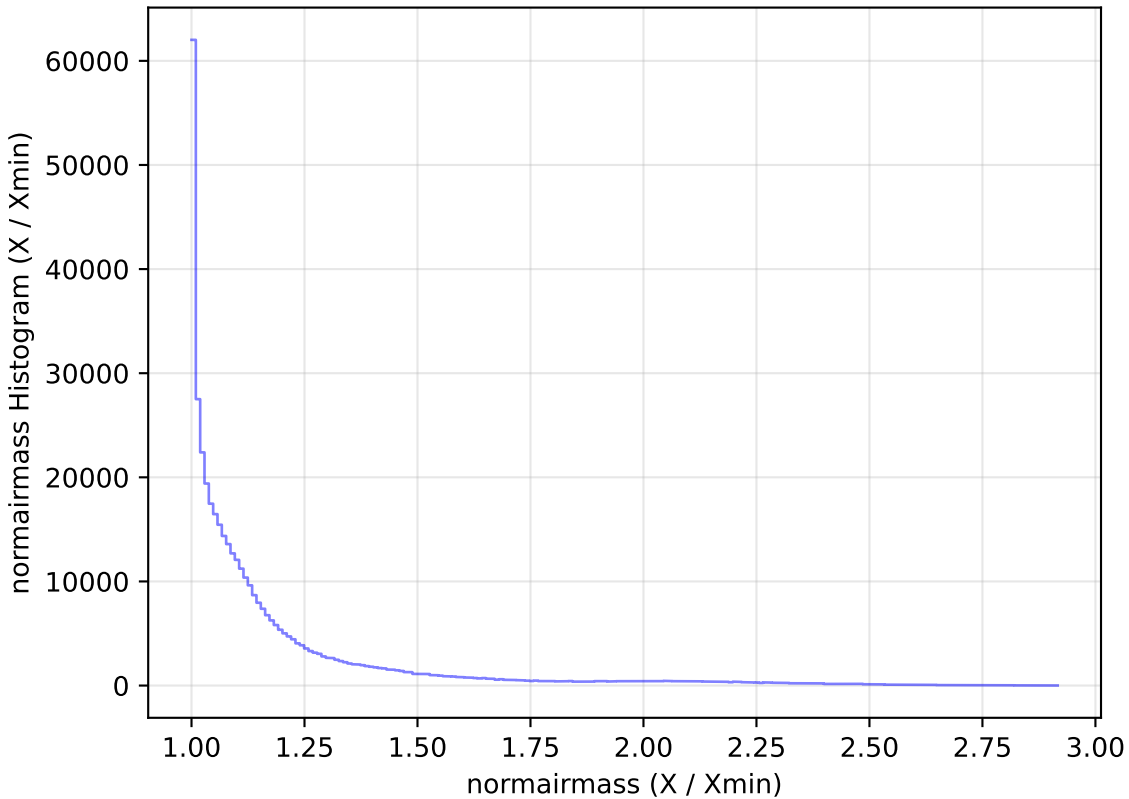
too_elab_r32_d2_gz_v3.4_10yrs WFD z band: normairmass Histogram
