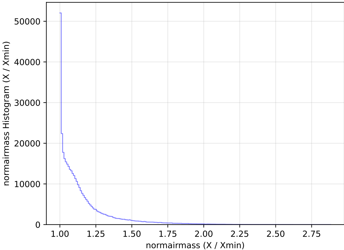
too_elab_r32_d2_gz_v3.4_10yrs WFD y band: normairmass Histogram
