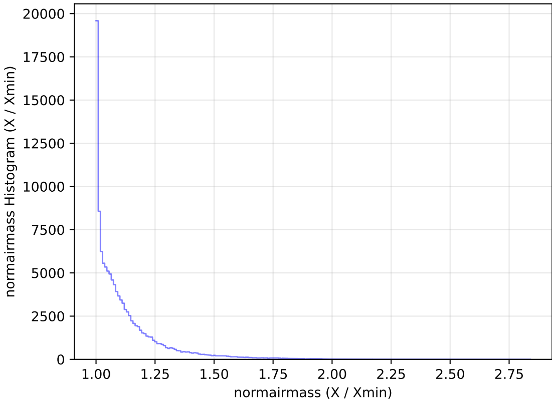
too_elab_r32_d2_gz_v3.4_10yrs WFD u band: normairmass Histogram
