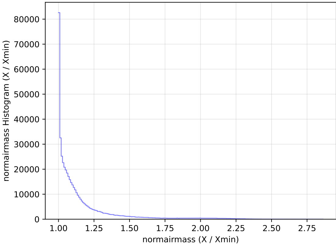
too_elab_r32_d2_gz_v3.4_10yrs WFD r band: normairmass Histogram
