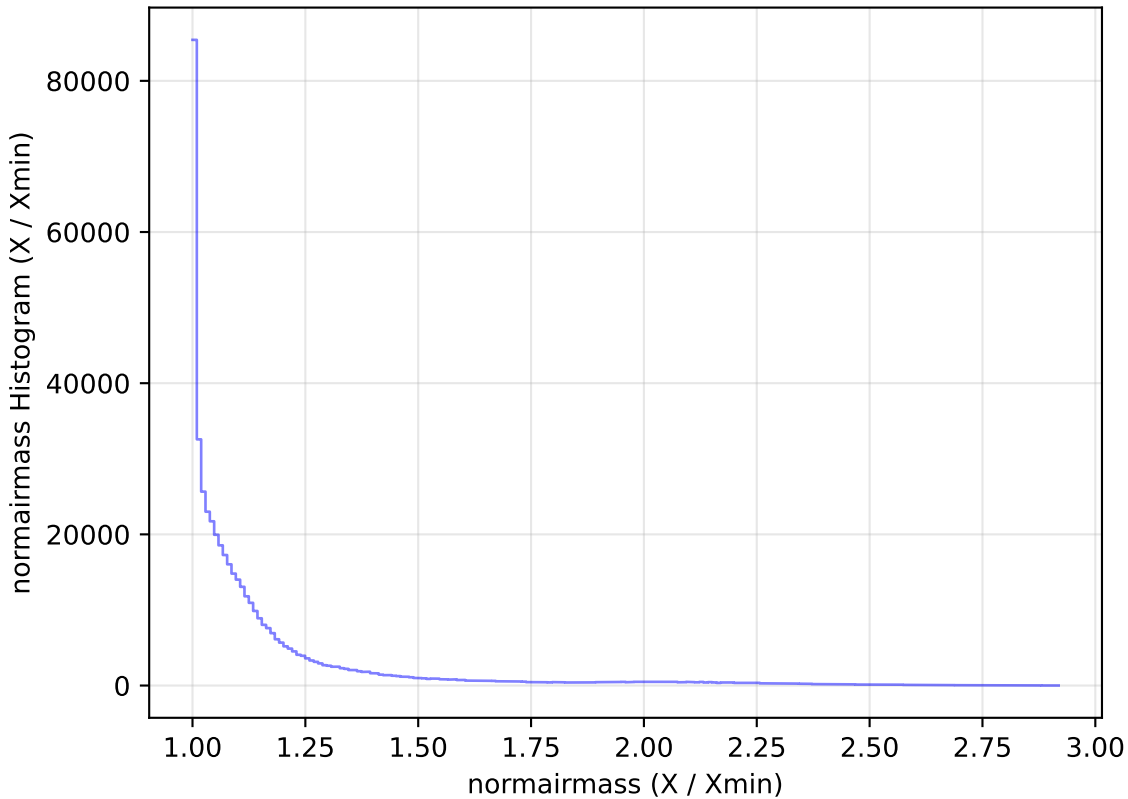
too_elab_r32_d2_gz_v3.4_10yrs WFD i band: normairmass Histogram
