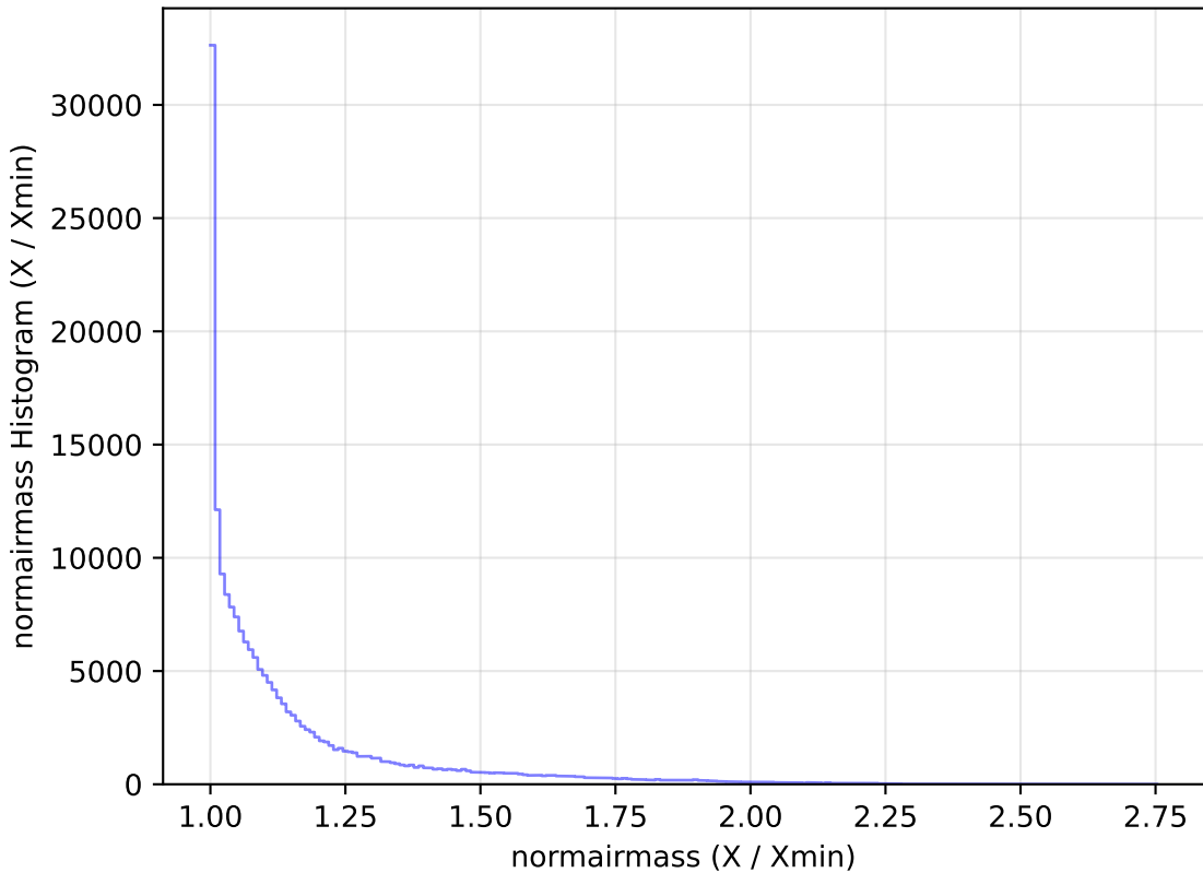
too_elab_r32_d2_gz_v3.4_10yrs WFD g band: normairmass Histogram
