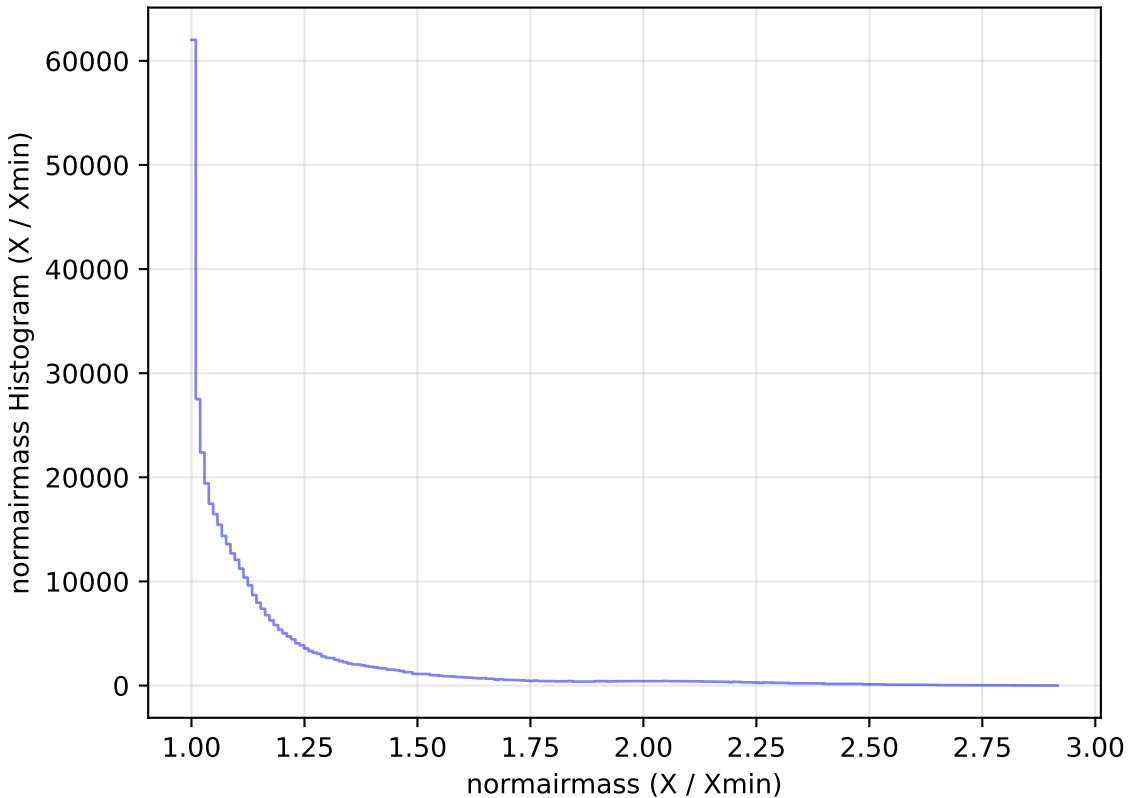
too_elab_r32_d2_gz_v3.4_10yrs All sky z band: normairmass Histogram
