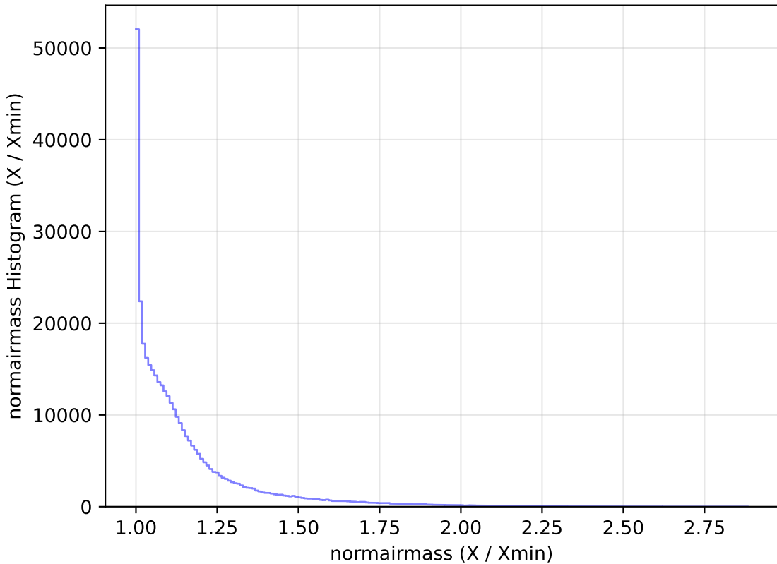
too_elab_r32_d2_gz_v3.4_10yrs All sky y band: normairmass Histogram
