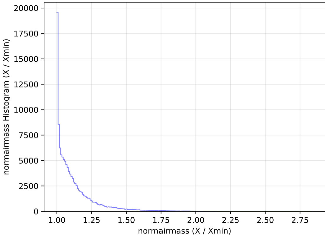
too_elab_r32_d2_gz_v3.4_10yrs All sky u band: normairmass Histogram
