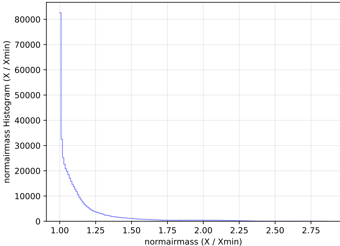
too_elab_r32_d2_gz_v3.4_10yrs All sky r band: normairmass Histogram
