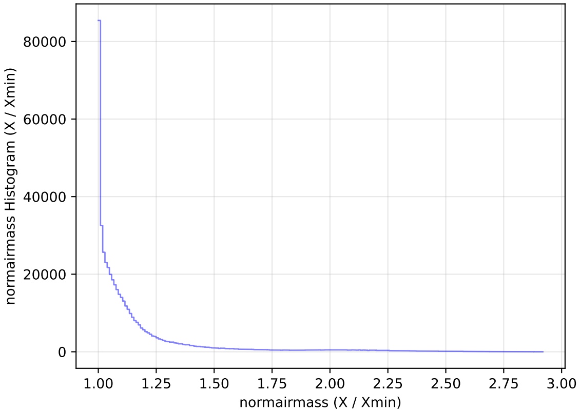
too_elab_r32_d2_gz_v3.4_10yrs All sky i band: normairmass Histogram
