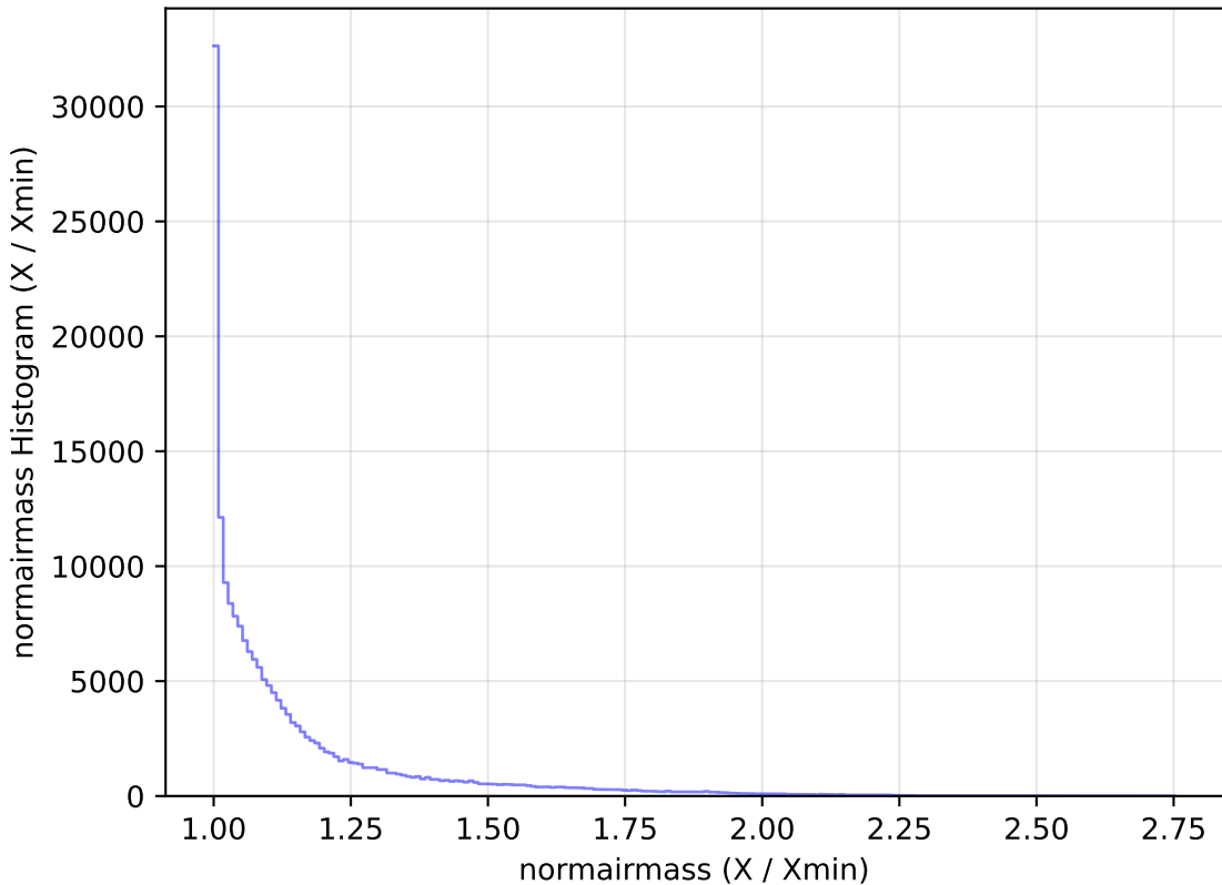
too_elab_r32_d2_gz_v3.4_10yrs All sky g band: normairmass Histogram
