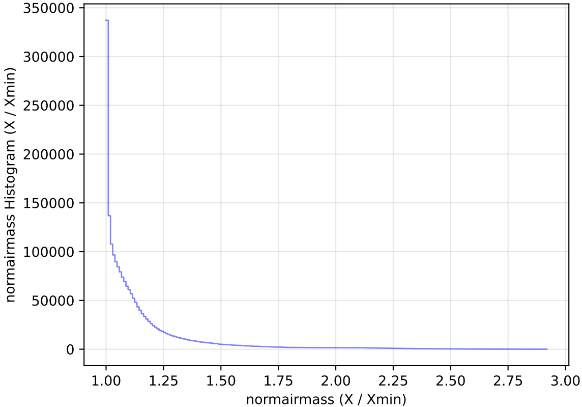
too_elab_r32_d2_gz_v3.4_10yrs All sky all bands: normairmass Histogram
