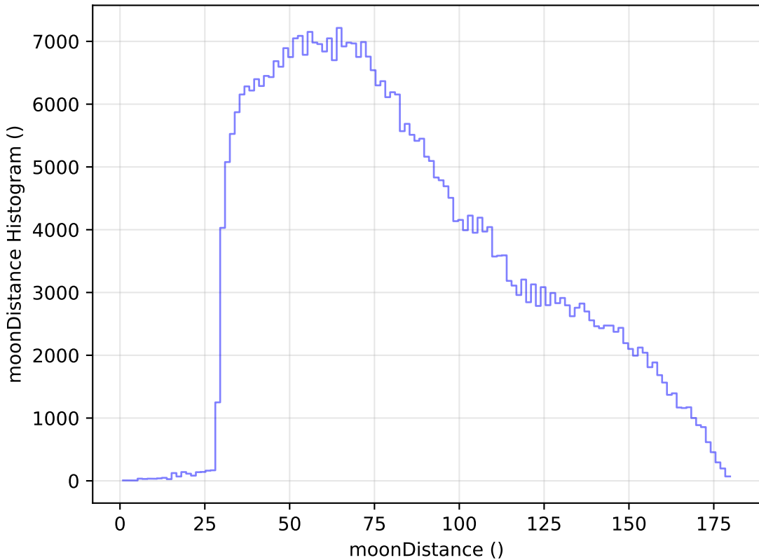
too_elab_r32_d2_gz_v3.4_10yrs WFD z band: moonDistance Histogram
