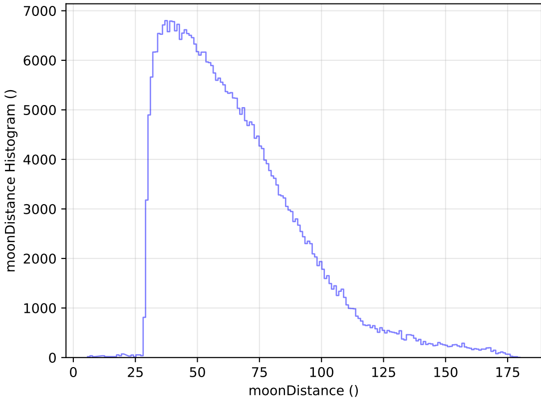
too_elab_r32_d2_gz_v3.4_10yrs WFD y band: moonDistance Histogram
