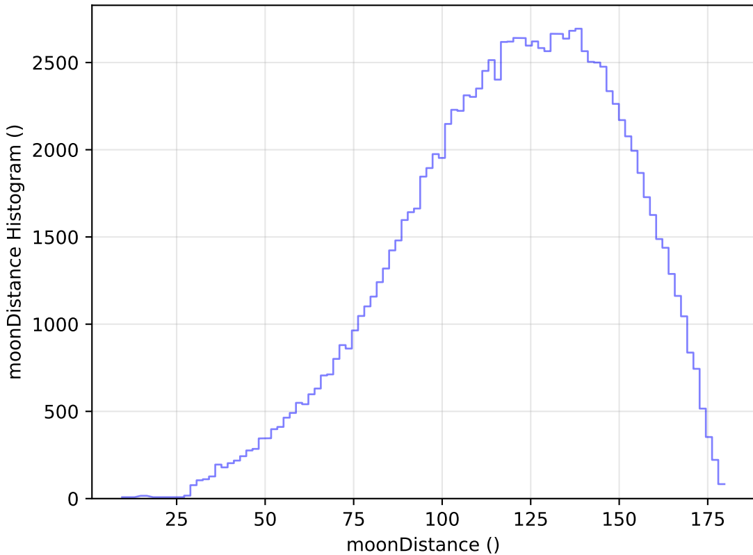
too_elab_r32_d2_gz_v3.4_10yrs WFD u band: moonDistance Histogram
