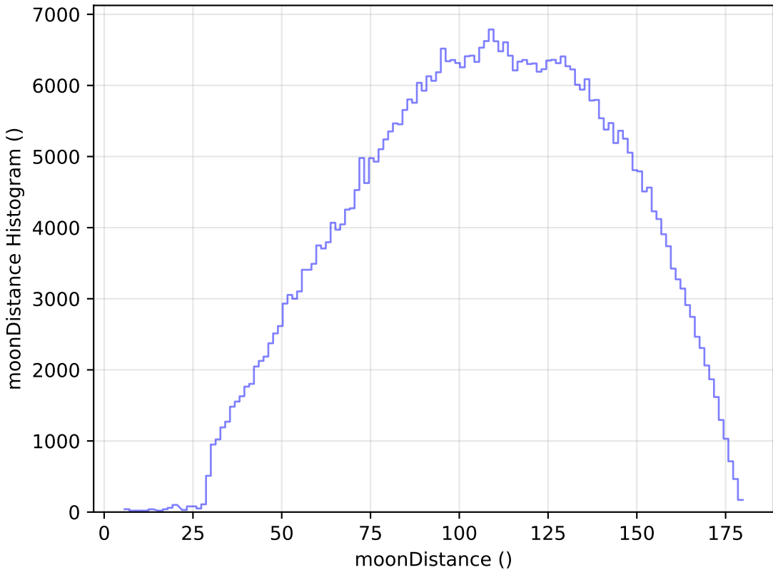
too_elab_r32_d2_gz_v3.4_10yrs WFD r band: moonDistance Histogram
